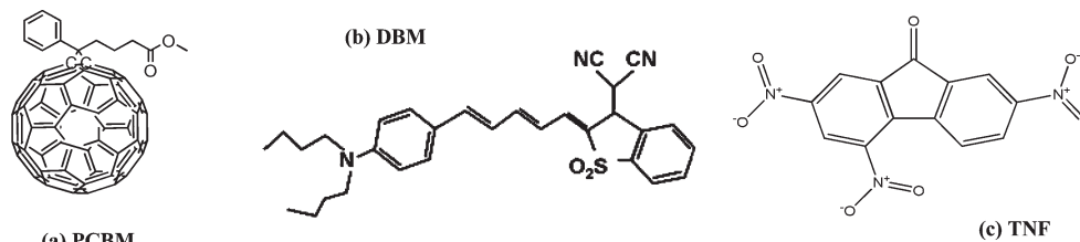
Figure 5. Typical sensitizer molecules. (a) [6,6]-Phenyl-C 61 -butyric acid-methylester (PCBM). (b) 2-[2-{5-[4-(Di- n -butylamino)phenyl]-2,4-pentadienylidene}-1,1-dioxido-1-benzothien-3(2H)-ylidene]malononitrile (DBM). (c) 2,4,7-Trinitro-9-fluorenone (TNF).
