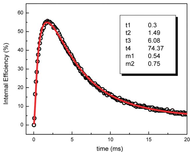
Figure 9. Simultaneous rise and decay of the diffraction efficiency under single pulse illumination. Pulse width was 1 ns and energy density was 4 mJ/cm 2 , applied field was 95 V/μm. Reproduced with permission from ref 109. Copyright 2006 American Institute of Physics.
