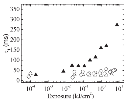
Figure 7. Dependence of fast time constant in transient FWM experiments on exposure. Open symbols are based on PATPD, filled triangles are based on PVK. Reproduced with permission from ref 31. Copyright 2004 Wiley-VCH.
