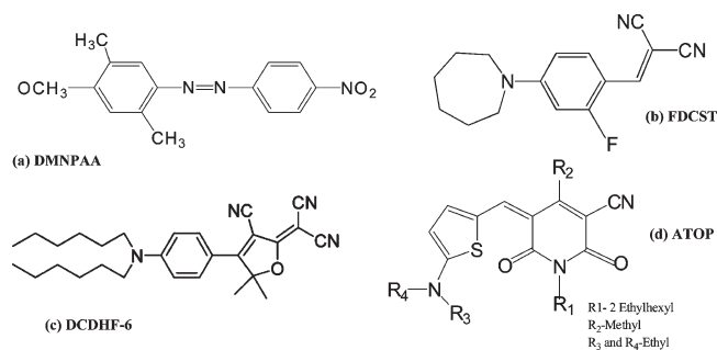
Figure 4. Some high-performing chromophores. (a) 2,5-Dimethyl-4-(p-phenylazo)anisole (DMNPAA). (b) Fluorinated dicyanostyrene 4-homopiperidino benzylidene malonitrile (FDCST). (c) 2-Dicyanomethylene-3-cyano-2,5-dihydrofuran (DCDHF-6). (d) Amino thienyl-dioxypyridine (ATOP).
