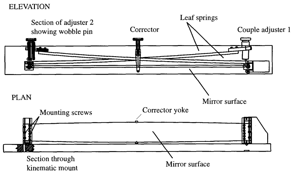
Fig. 3. Mechanical layout of the mirror substrate and its bending mechanism
