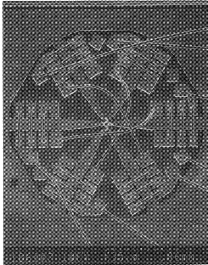
Fig. 6 Integrated magnetic variable reluctance micromotor with shaft encoder. A bonded coil implementation was used here. The rotor and stator are fabricated from electroplated 78 Permalloy. Metallization runners to the shaft encoder underneath the 150 \mu m diameter rotor are apparent.
