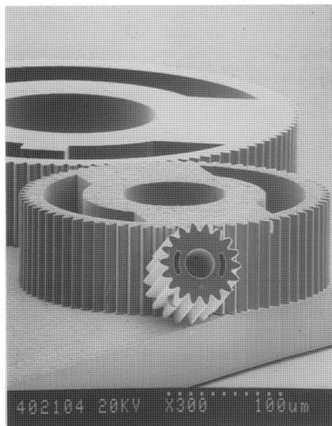
Fig. 4 SEM photograph of released nickel gears fabricated by DXRL and electroplating. The smallest gear has a 70 \mu m diameter with 100 \mu m thickness.
