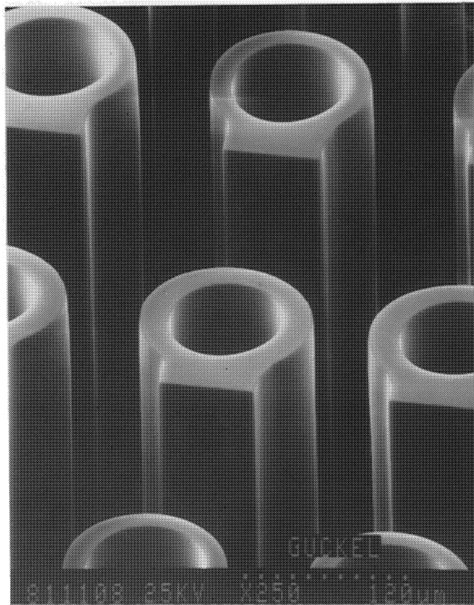
Fig. 2 Developed PMMA test structures 3.2 mm thick exposed with 2.5 GeV synchrotron radiation at the National Synchrotron Light Source of Brookhaven National Laboratory.
