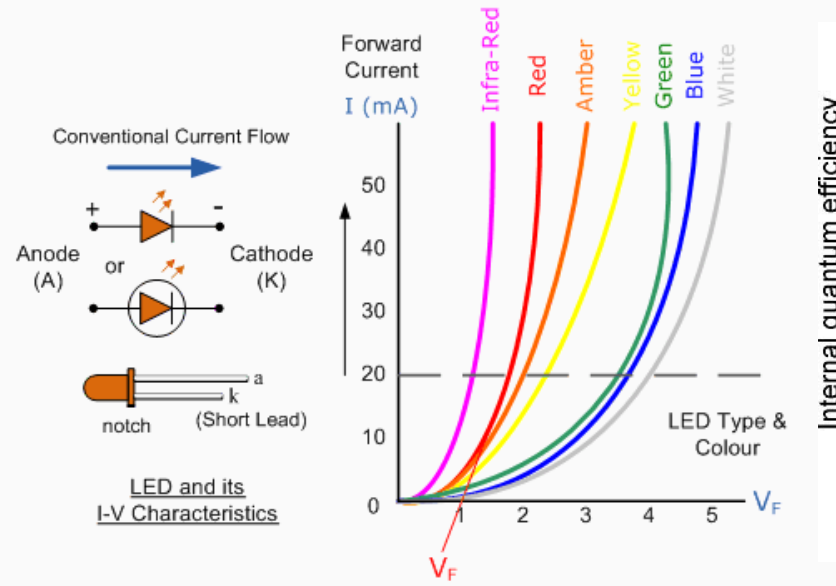
Light Emitting Diodes I-V Characteristics.
