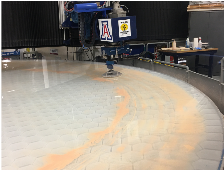
Figure 1. GMT Segment 3 being polished with a 40 cm pitch lap on an orbital polisher.
