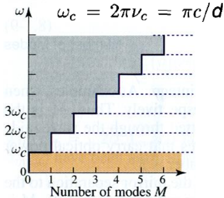
Mirror waveguide
