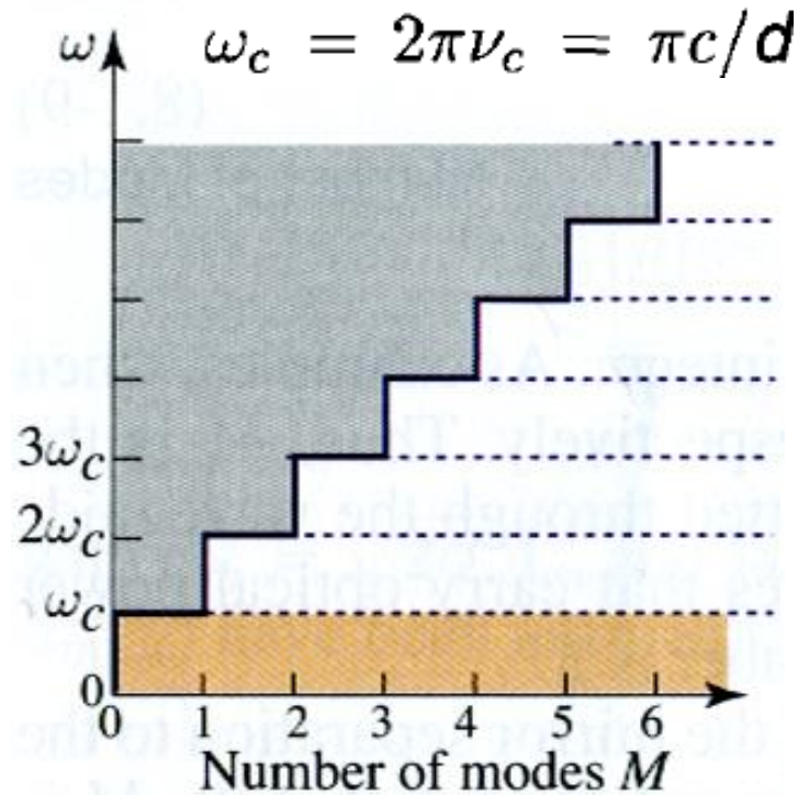
Mirror waveguide
