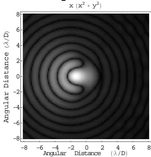
Point Spread Function
