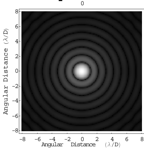
Point Spread Function
