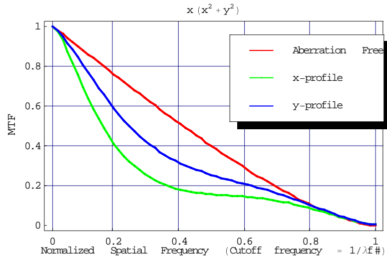
Modulation Transfer Function
