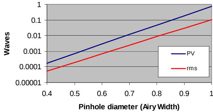
Figure 5. Calculated wavefront error of synthetic reference wave as a function of pinhole diameter (relative to Airy width of focused beam).
